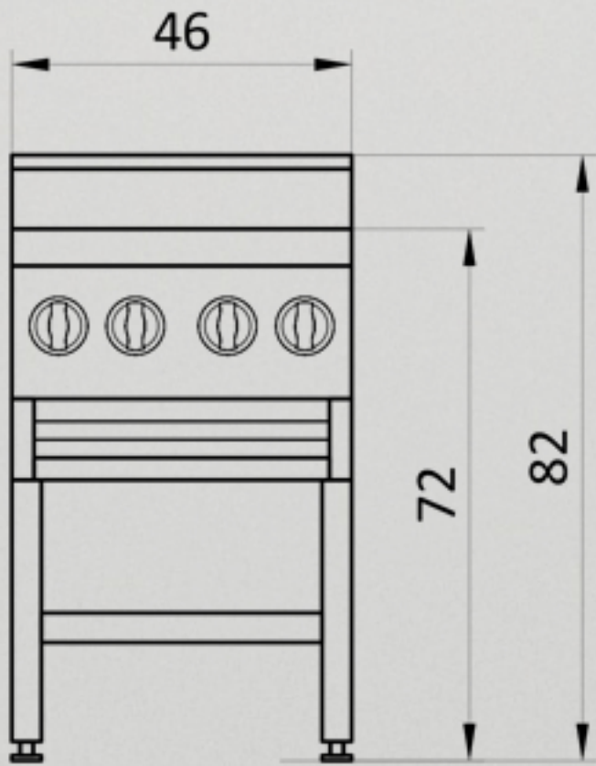
VISTA FRONTAL
