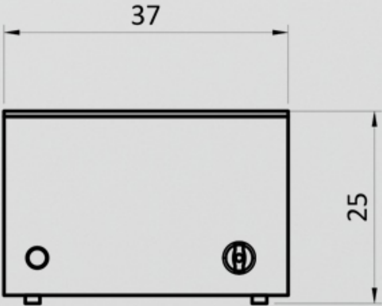
VISTA FRONTAL
