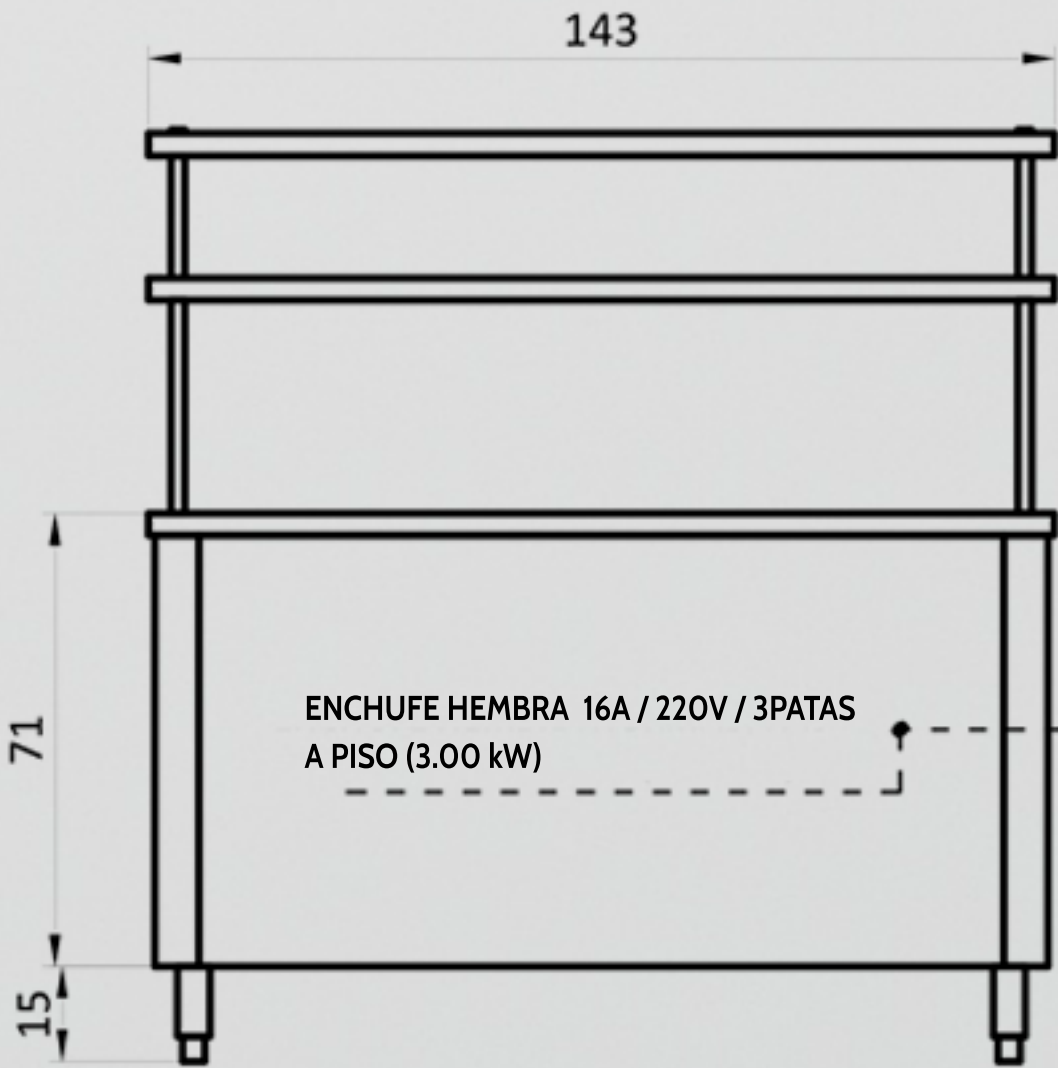
VISTA FRONTAL
