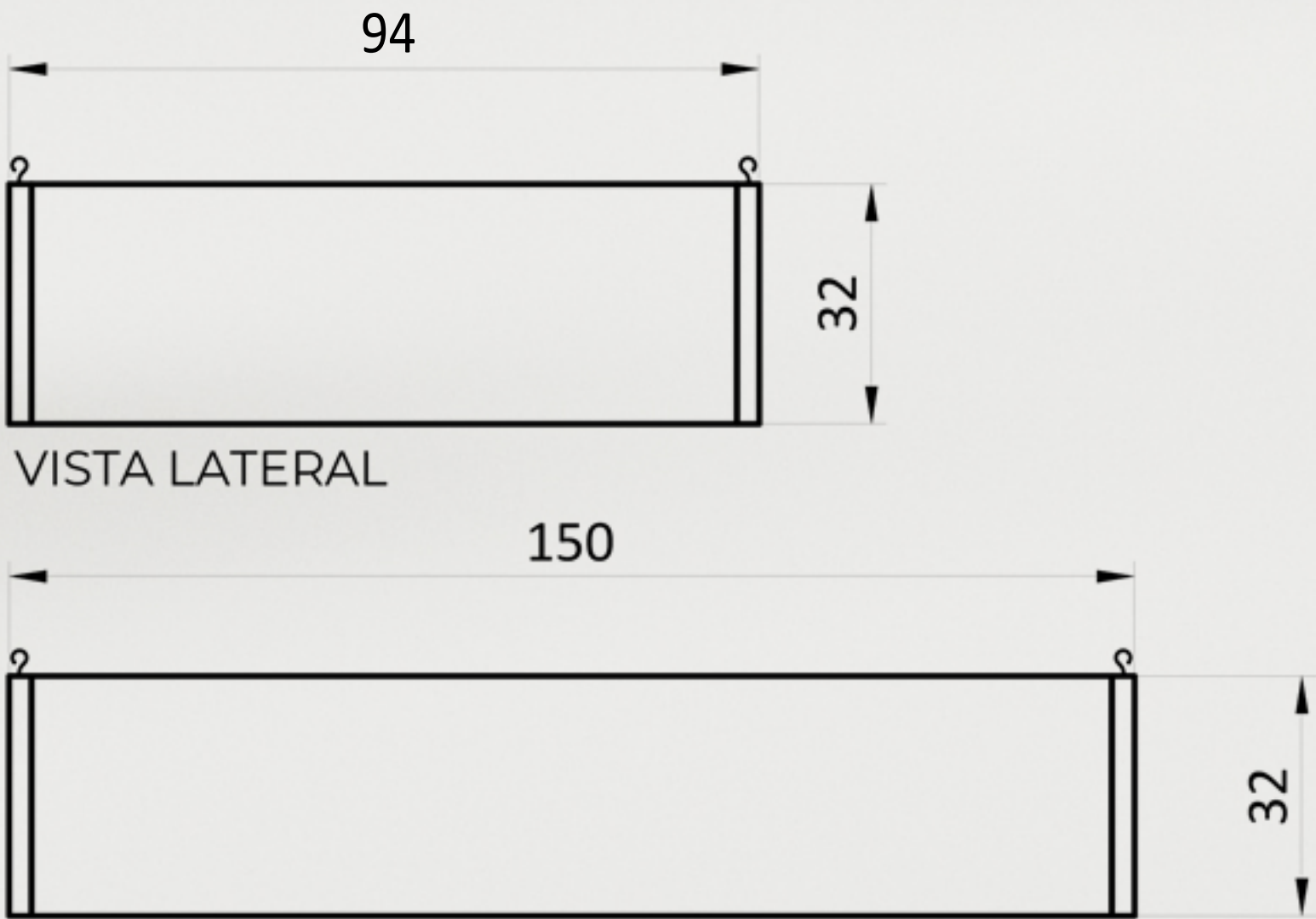
VISTA FRONTAL
