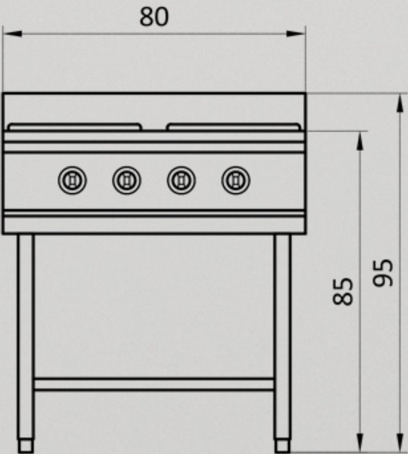
VISTA FRONTAL
