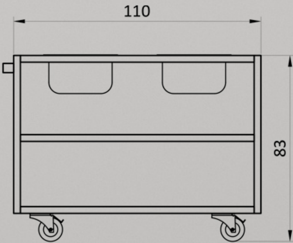
VISTA FRONTAL
