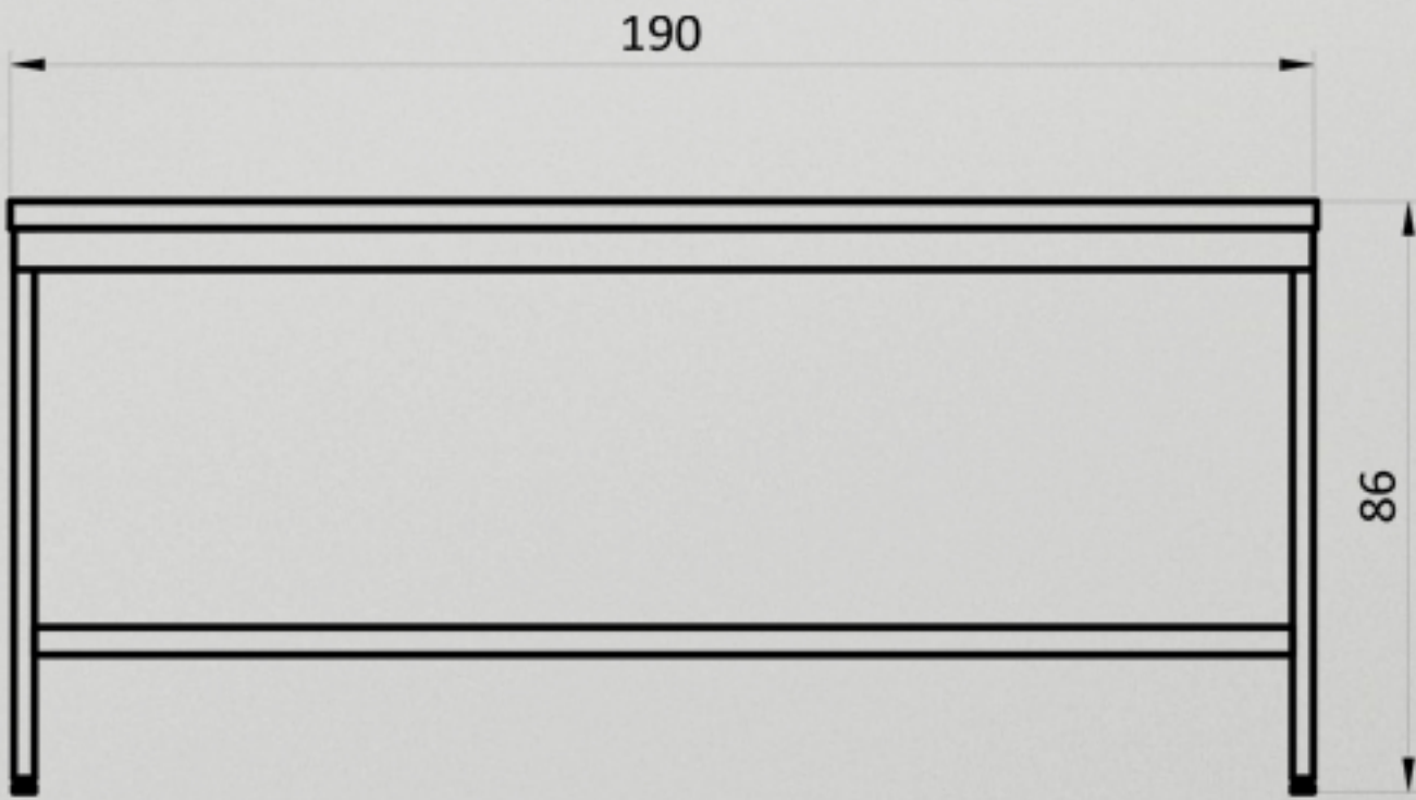
VISTA FRONTAL
