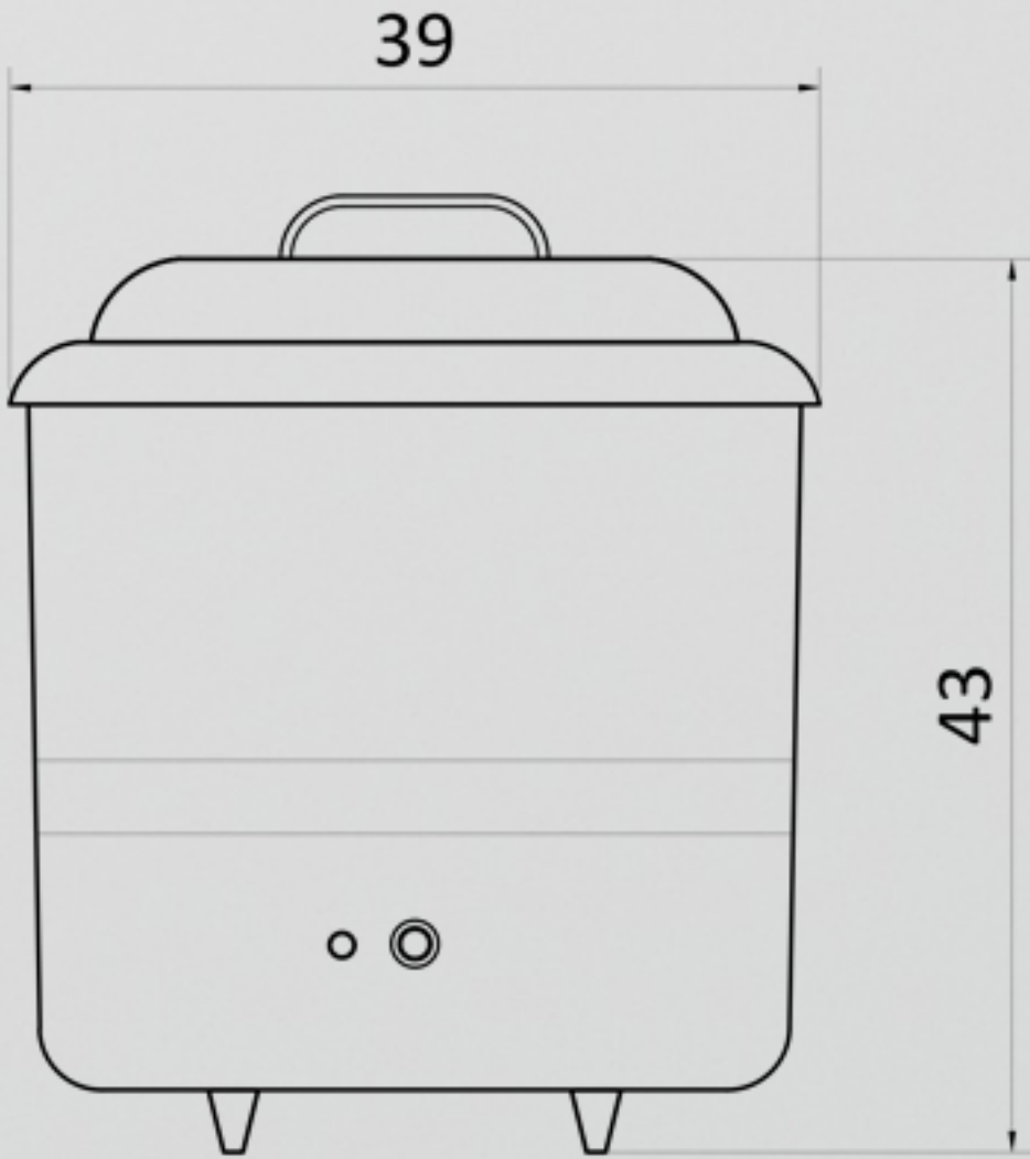
VISTA FRONTAL
